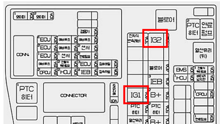
Engine room fuse box
